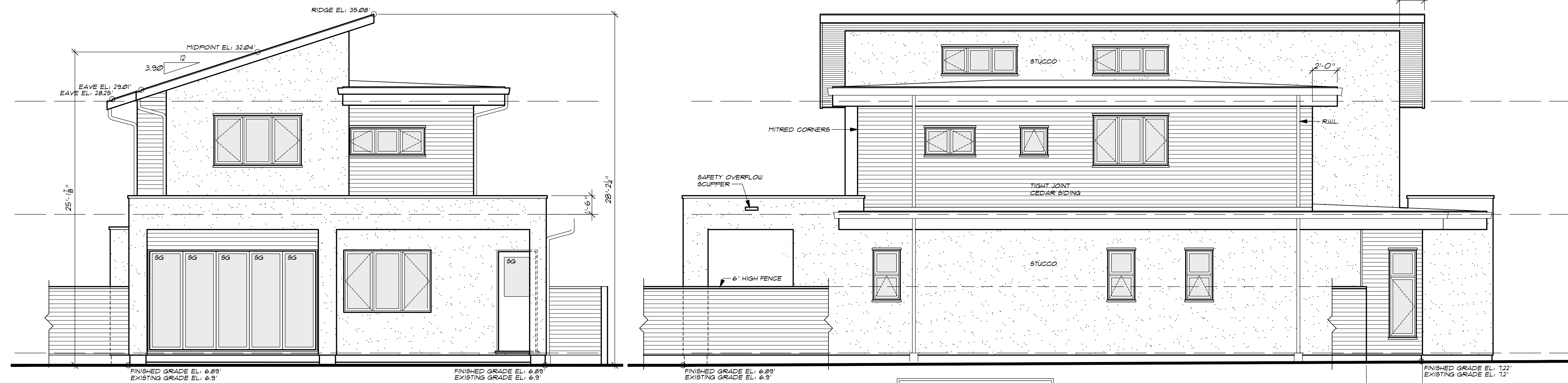
rear elevation
